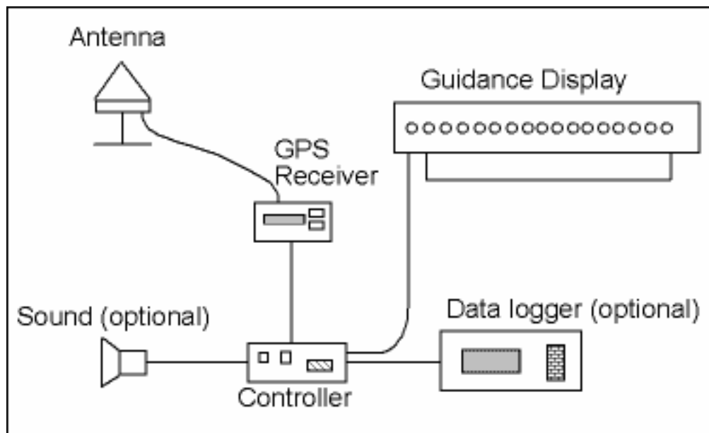
Figure 1. Components of a guidance system.
